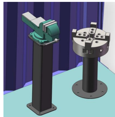
Vice and flange chuck
